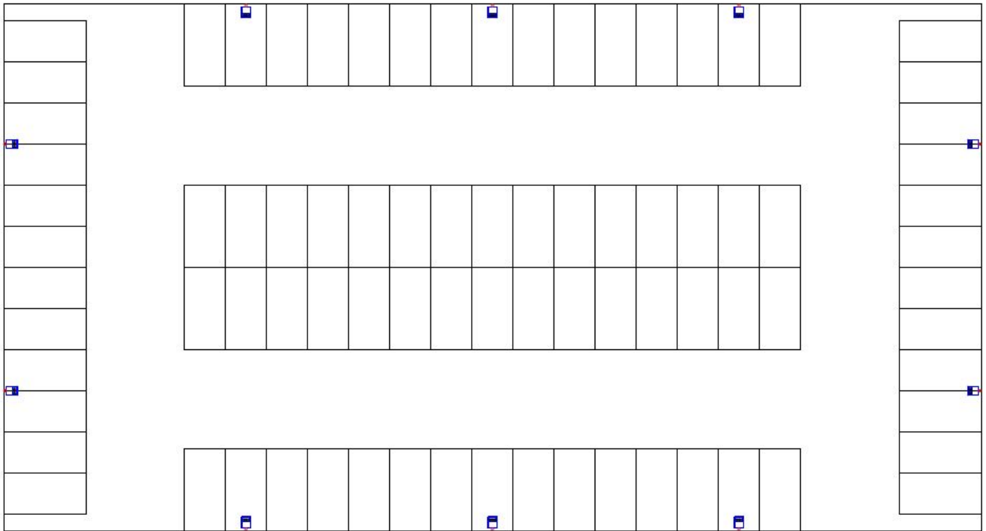
Standard proposal Private (Public) Outdoor car park to the standard NEN-EN 12464-1:2021
